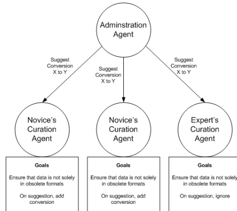
Fig. 7. An agent-oriented design of the data curation tool
